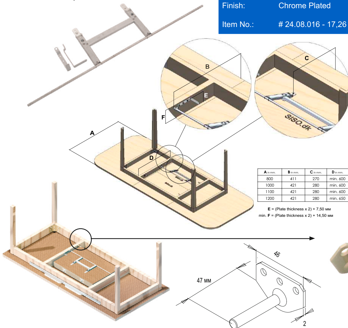
Hide Away Mechanism for Folded Table Tops seen from bottom with other accessories mounted
